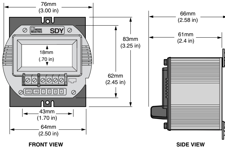
Figure 5. Dimensions of SDY Hockey-Puck with Flange Mount
